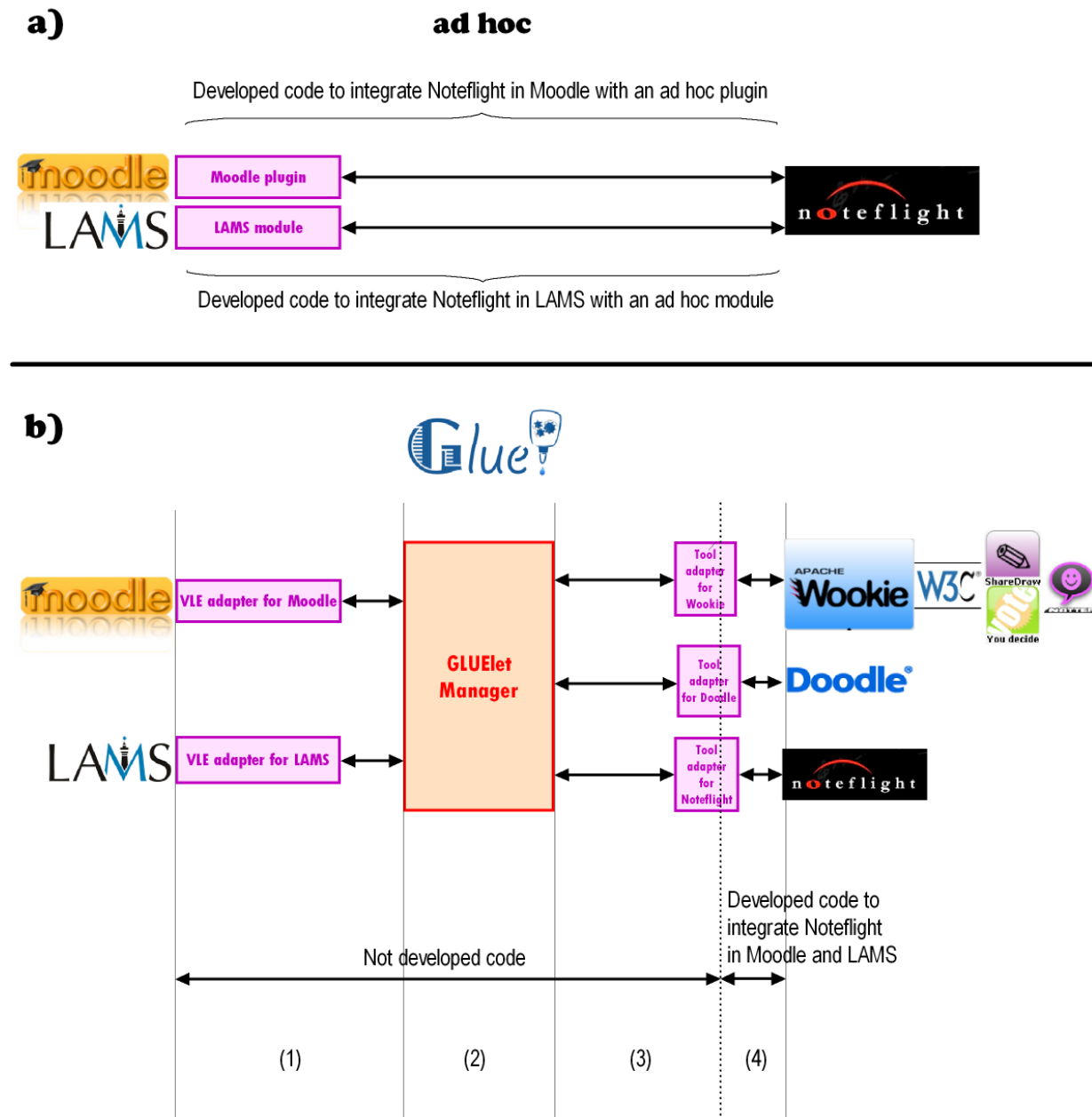
Figure 5.5: Examples of the new SLOC in the integration of Noteflight in Moodle and LAMS: a) without GLUE!; b) with GLUE!. The lower effort demanded with GLUE! is due to: (1) a three-layer architecture that promotes a many-to-many integration, allowing to reuse all the VLE-specific integration code encapsulated in VLE adapters; (2) a three-layer architecture that allocates most of the integration logic in a central element, which is reused for any integration; (3) standardized, simple and loosely-coupled contracts, which allow tool adapters to reuse the code that implements the communication with the GLUElet Manager. Only (4), the part of the tool adapter that implements the tool-specific contract, must be developed.
