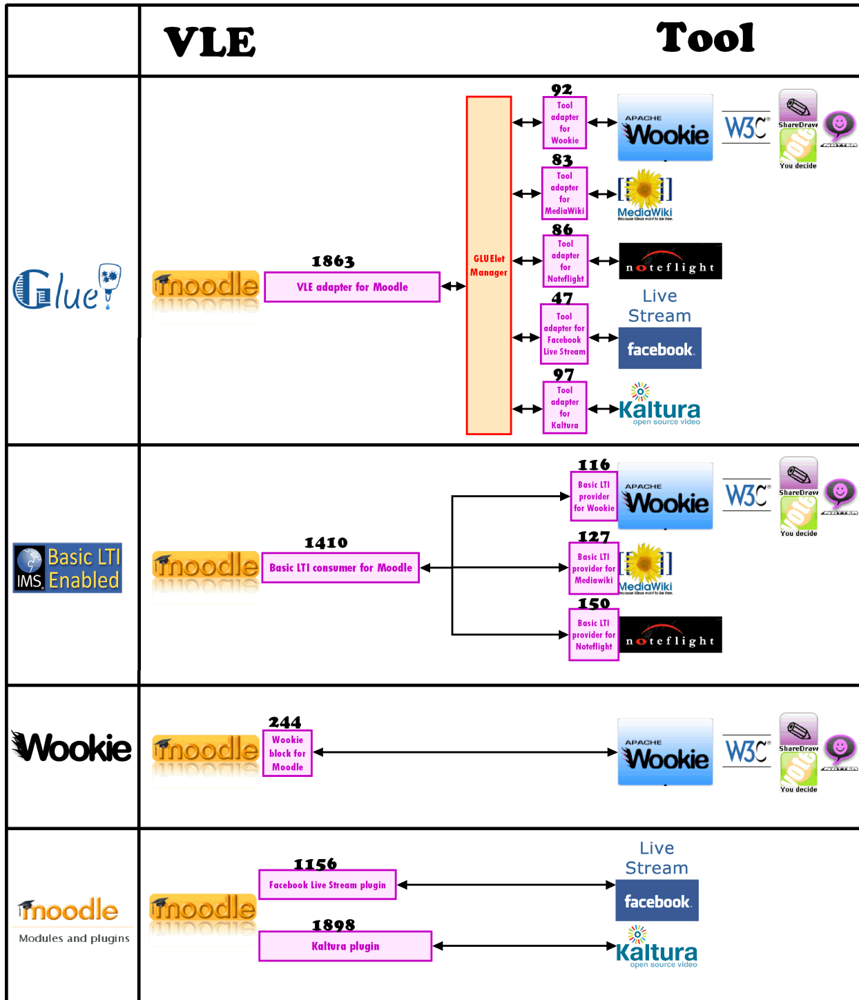
Figure 5.6: Examples of the new SLOC in loosely-coupled integration approaches: GLUE!, Basic LTI, Apache Wookiee and Moodle plugins.
